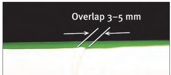
Figure 16: Adhering the two edges of the tape
