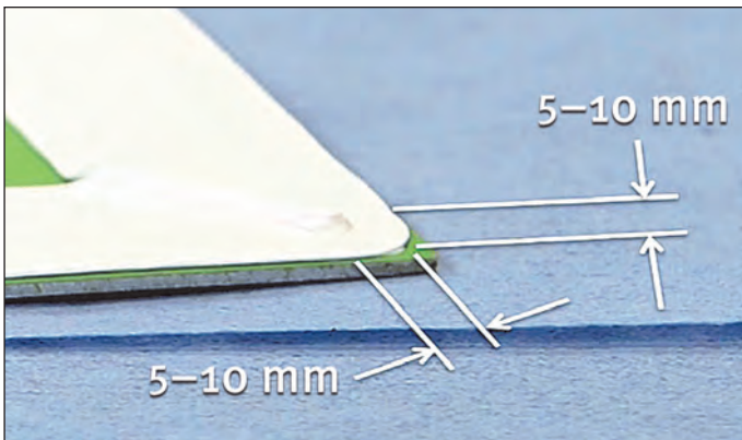
Figure 14: Sealing the tape around corner
